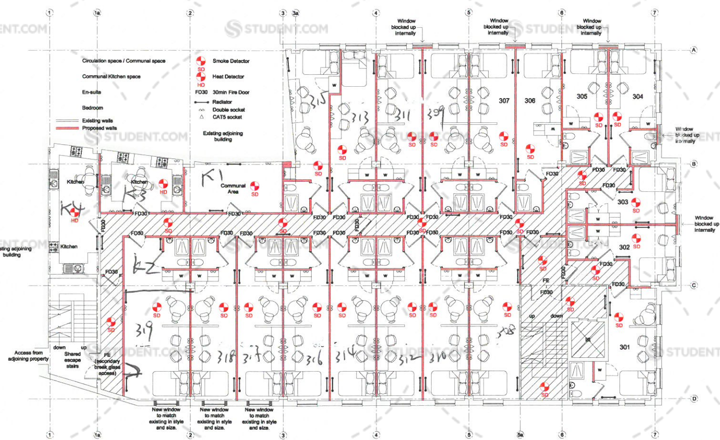
Third Floor Plan 19 Number Bedrooms (Inc 1 double) 1:100 @ A1
