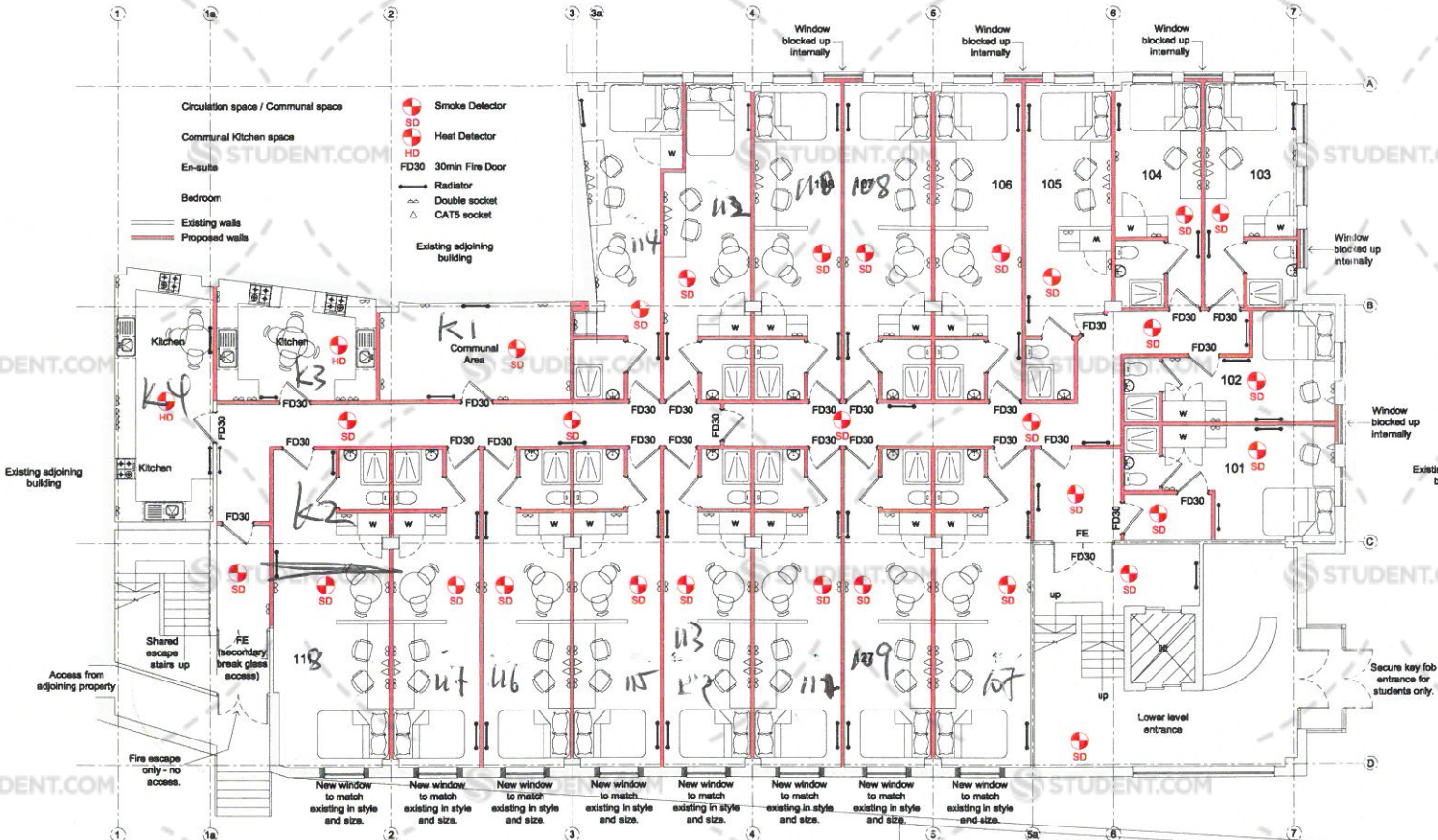
Entrance / First Floor Plan 1:100 @ A1
