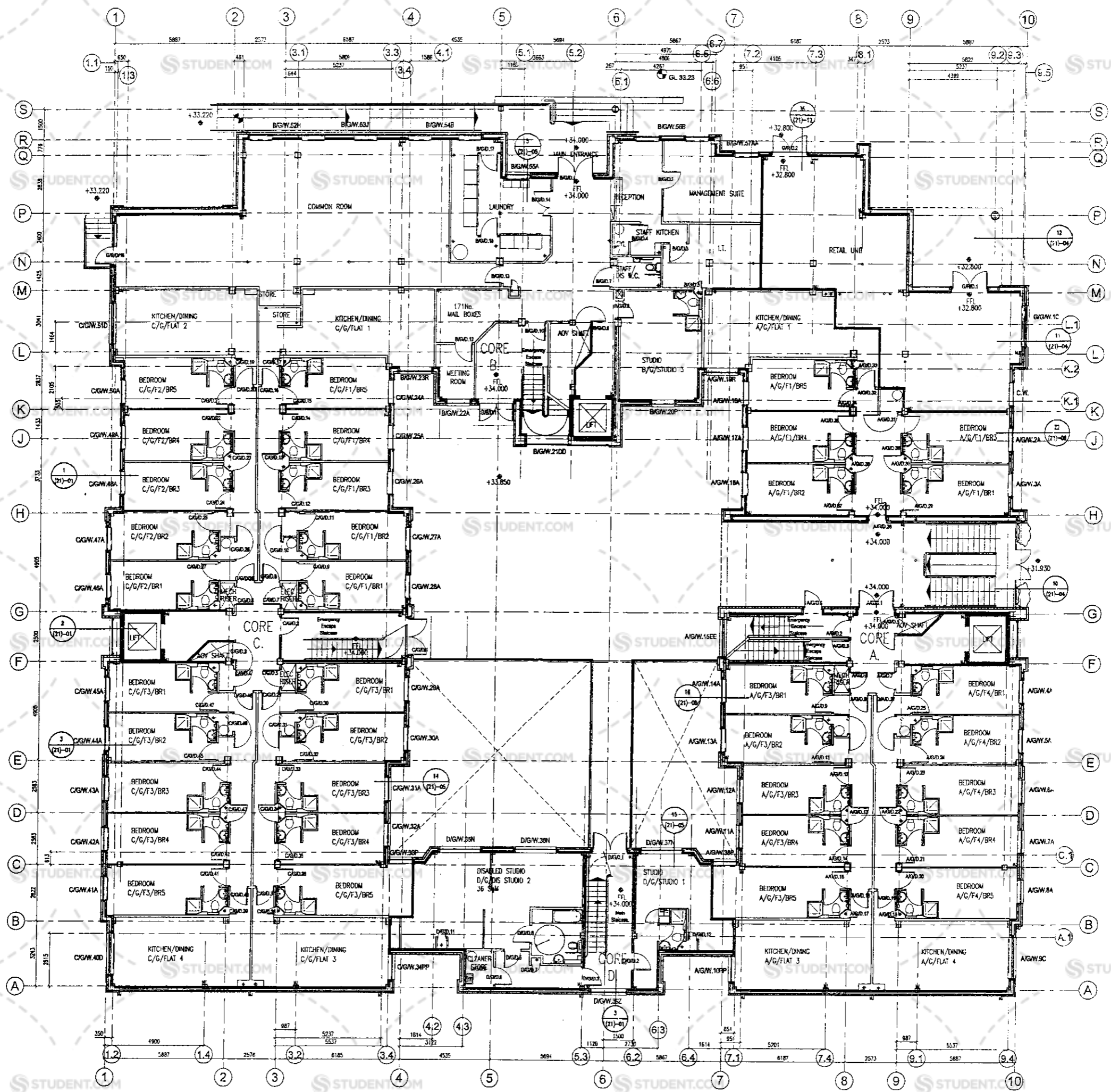
General Arrangement - Ground Floor Plan
