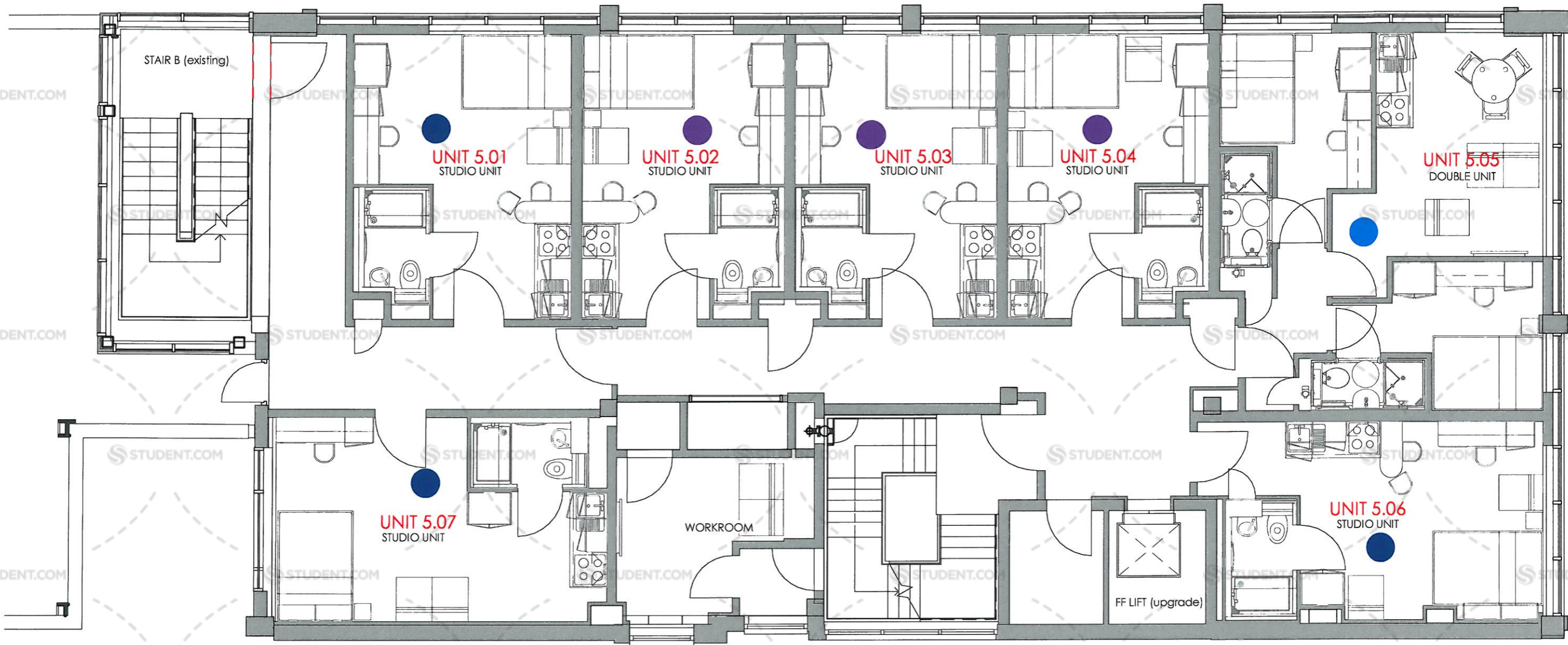
Block A - Fifth Floor Plan 1:100 @ A4
