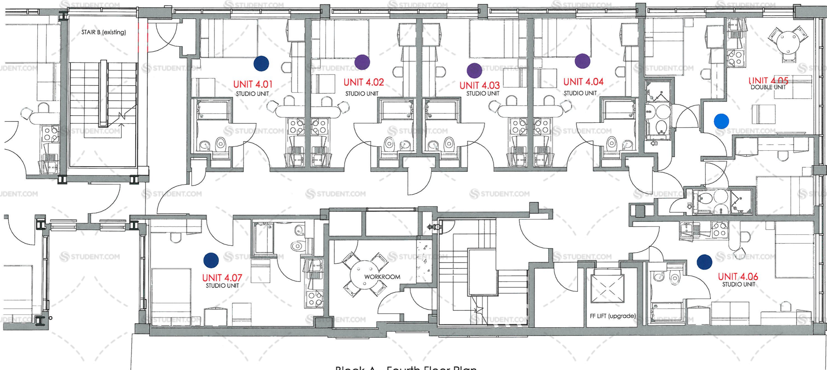
Block A - Fourth Floor Plan 1:100 @ A4
