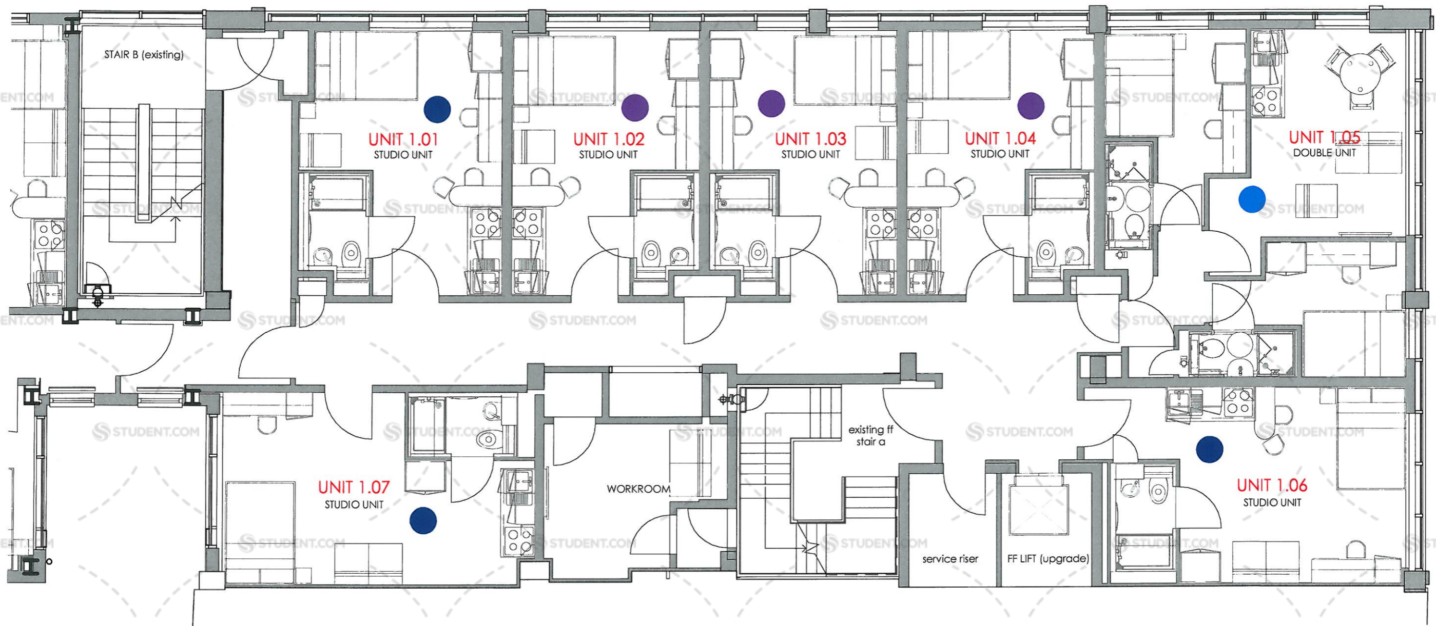
Block A - First Floor Plan 1:100 @ A4
