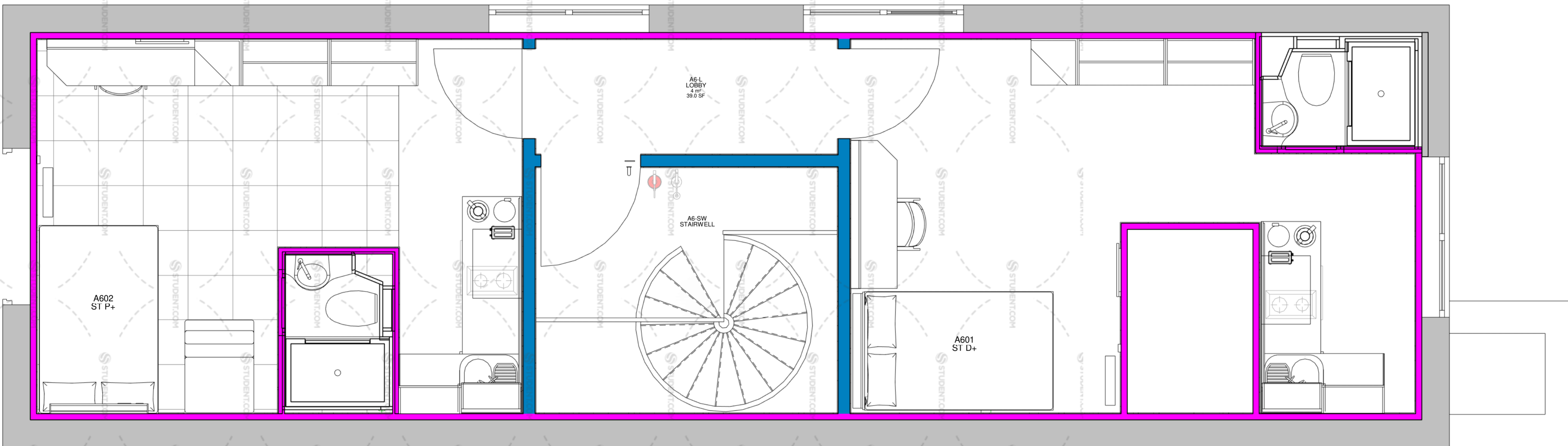
1 Level 6 MARKETING PLAN 1 : 25
