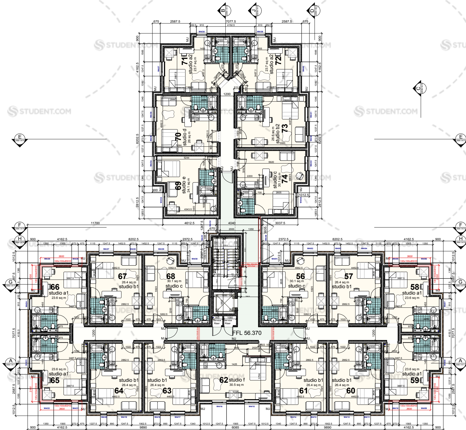
Level 04 Floor Plan
