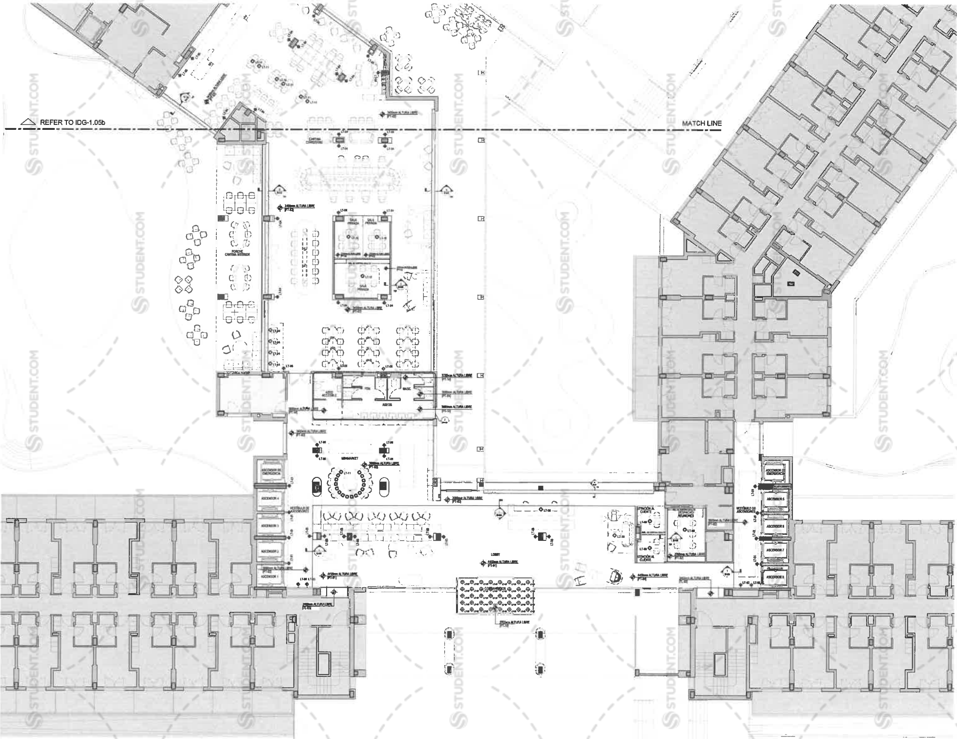
Reflected Ceiling - Planta baja
