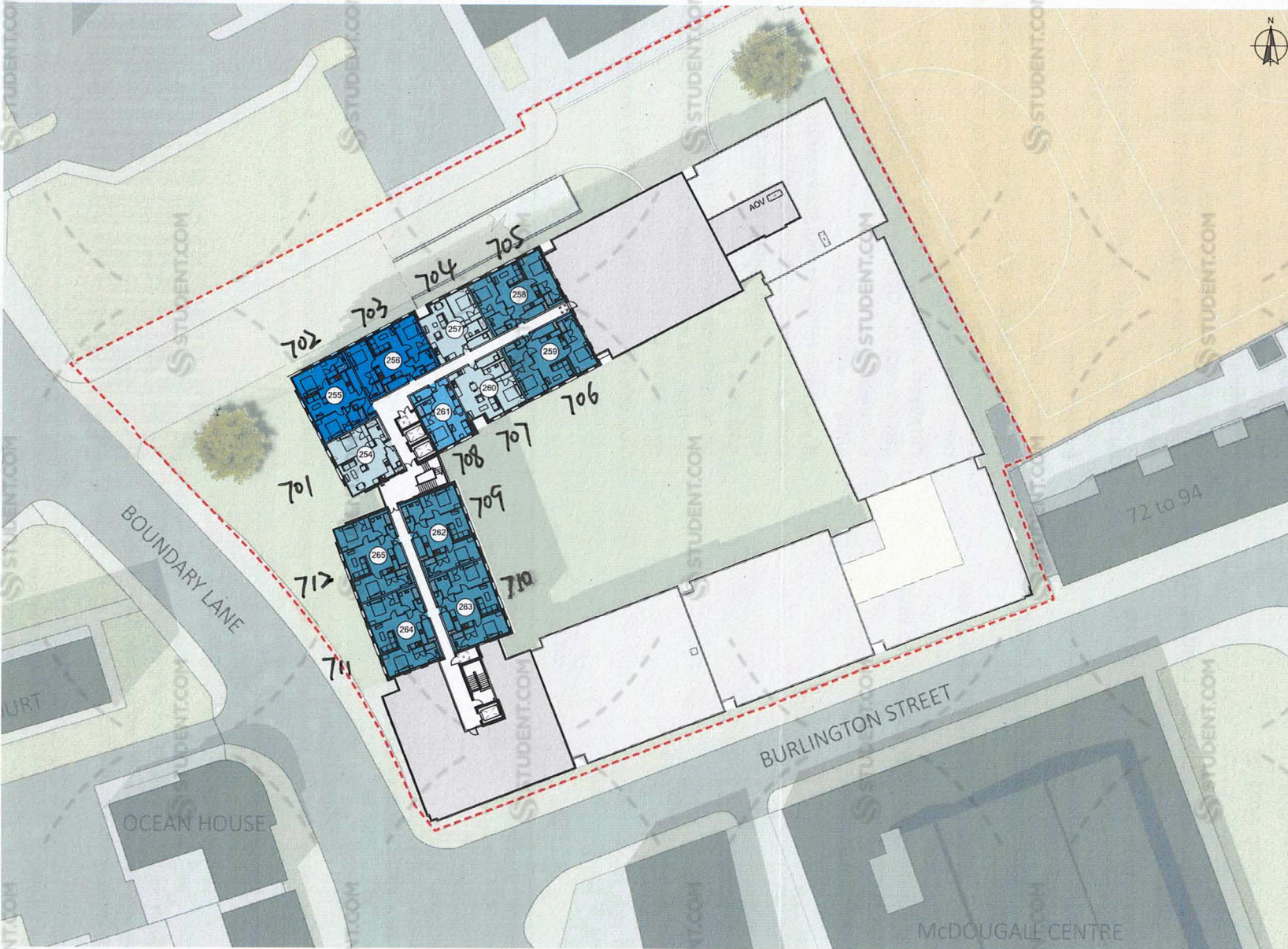
Level 07 - Seventh Floor Plan 1 : 500
