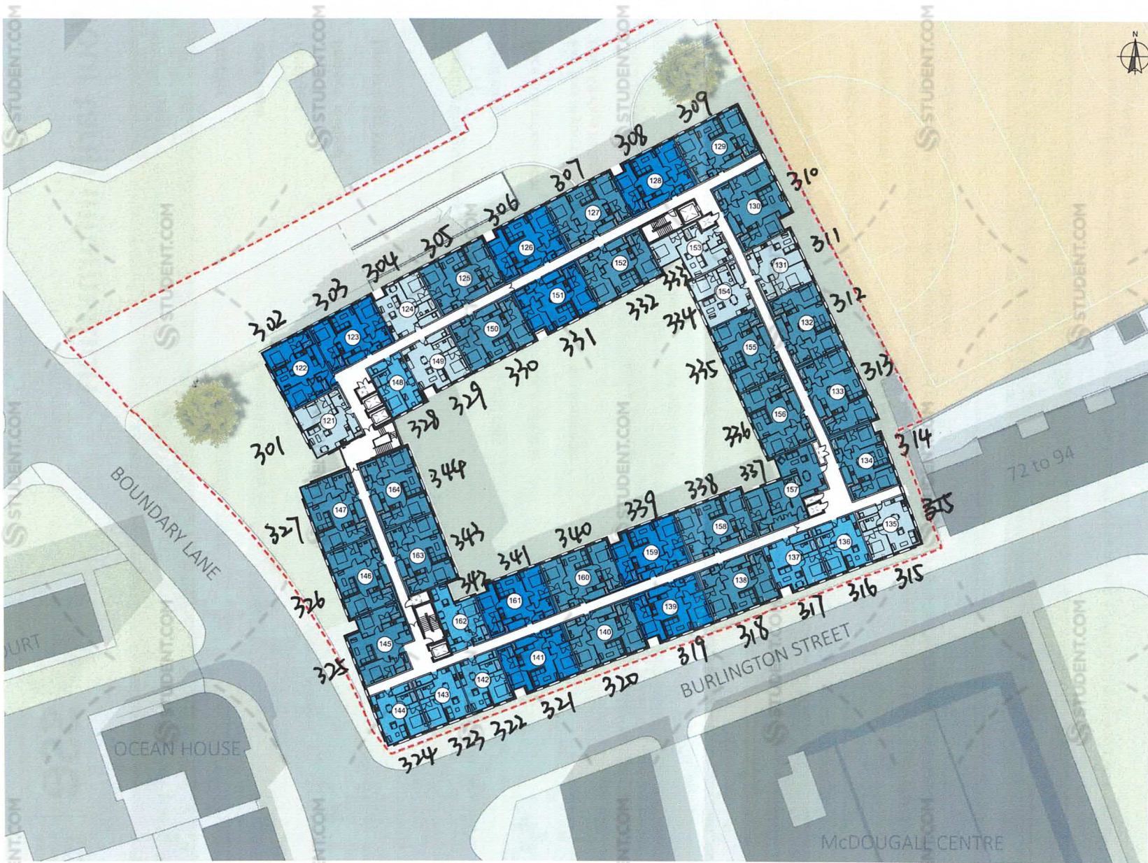
Level 03 - Third Floor Plan 1 : 500
