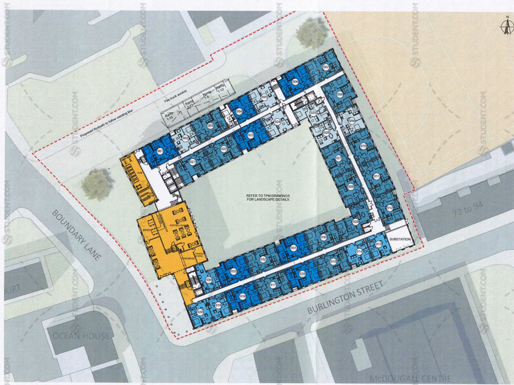
Level 00 - Ground Floor Plan 1 : 500
