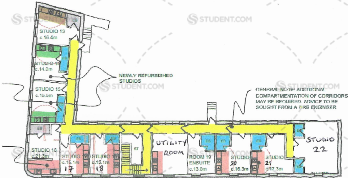
FIRST FLOOR
