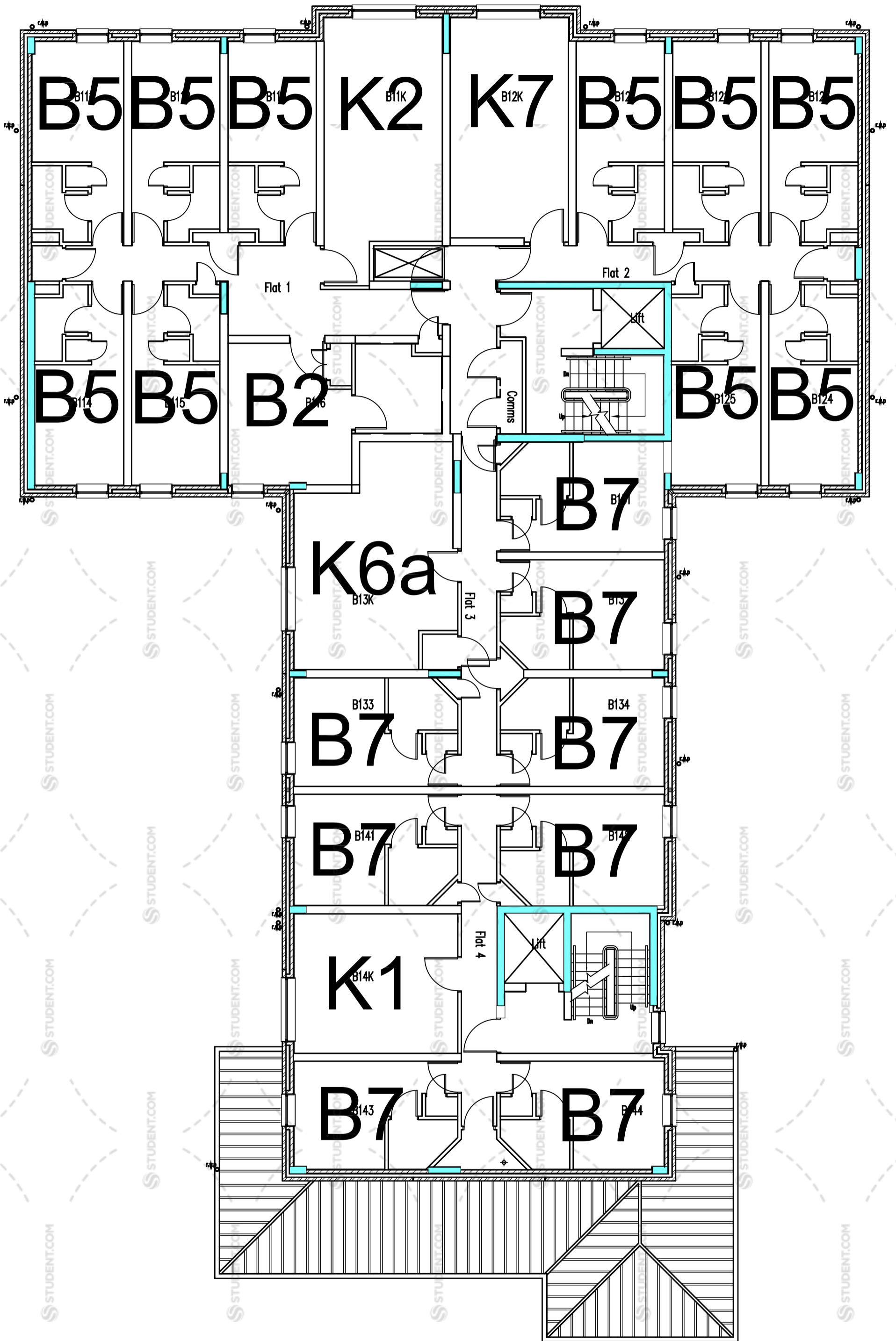
02 Typical Upper Floor Plan Scale 1:100@A1 Floors 01 - 02 layout repeats (First Floor shown).
