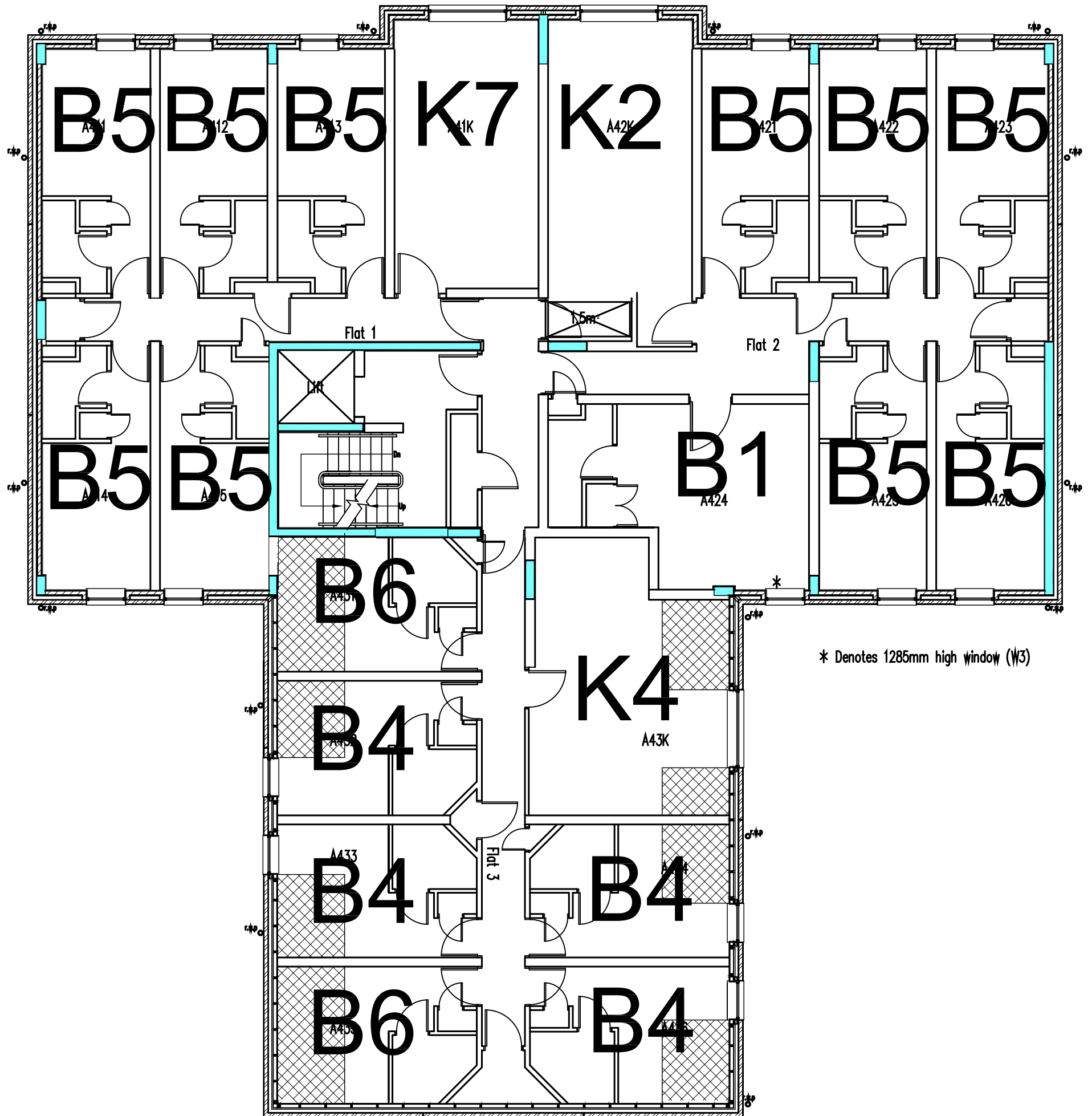
03 Fourth Floor Plan Scale 1:100@A1
