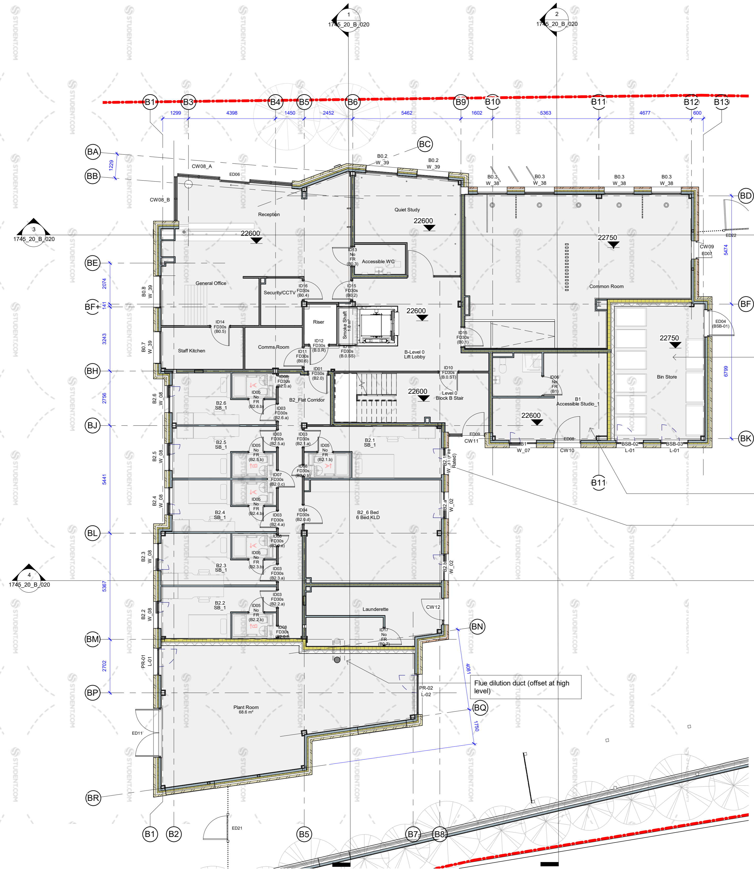
Block B _ Level 0 Plan View 1 : 100
