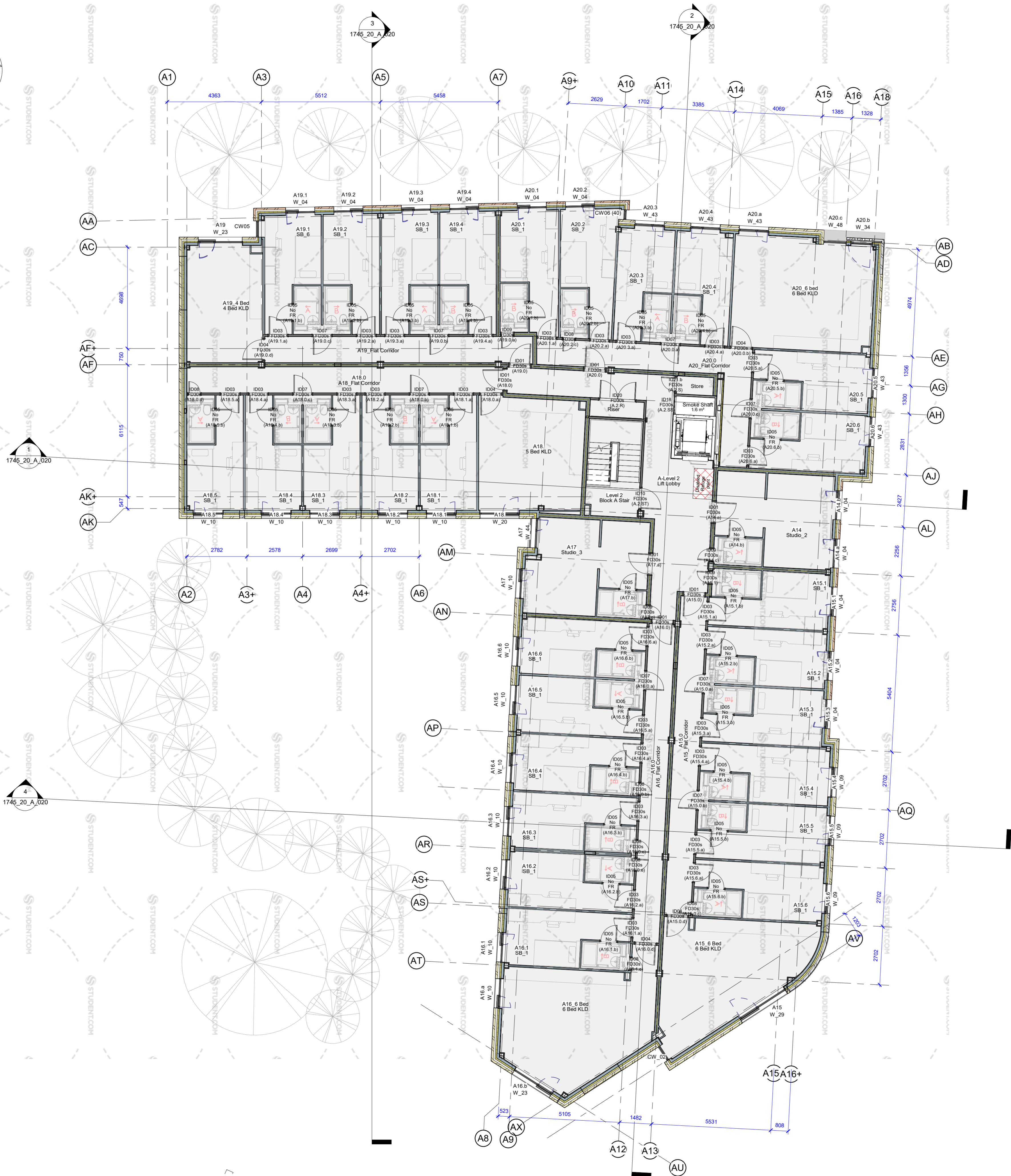
Block A _ Level 2 Plan View 1 : 100
